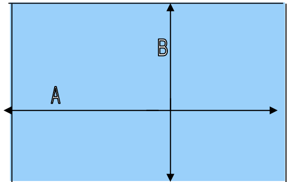
Rectangle
